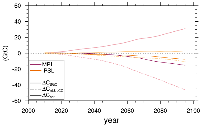
Fig. S5. 10-years-running global means of net changes due to LULCC in cumulative fire emissions of ESM runs (in GtC).
